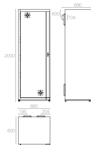
BC 650 S -External dimensions (LxDxH): 700x600x2015 mm -Internal dimensions (LxDxH): 445/403x548x1787 mm -Weight: 212 Kg -Storage capacity: ~435 lt
