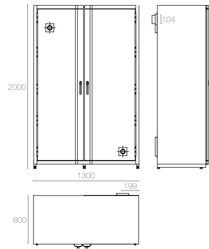
BC 1350 GS -External dimensions (LxDxH): 1300x600x2000 mm -Internal dimensions (LxDxH): 1165x500x1845 mm -Weight: 460 Kg -Storage capacity: ~1088 lt
